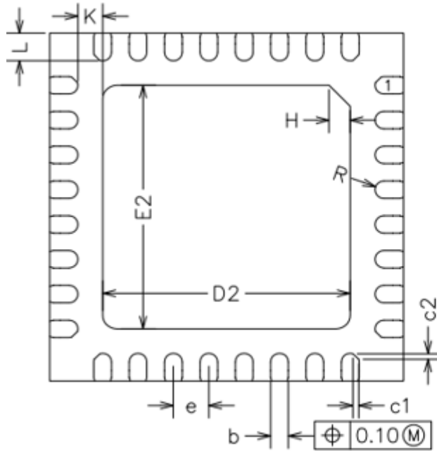
BOTTOM VIEW
